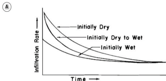
Fig. 5 Schematic Representation of the Effect of Soil Moisture on Infiltration Rates
